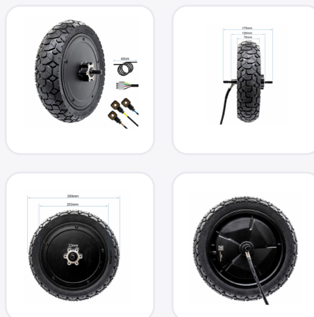
Motor views and dimensions
