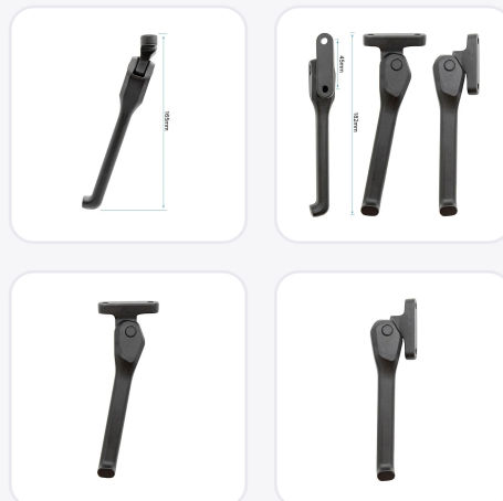
Kickstand views and dimensions
